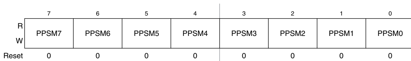
Figure 2-40. Port M Polarity Select Register (PPSM)
